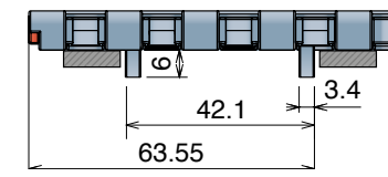
Version C - 2 Positioner
