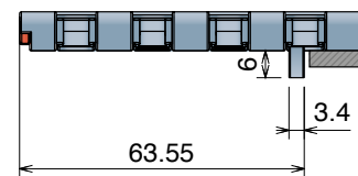
Version B - 1 Positioner
