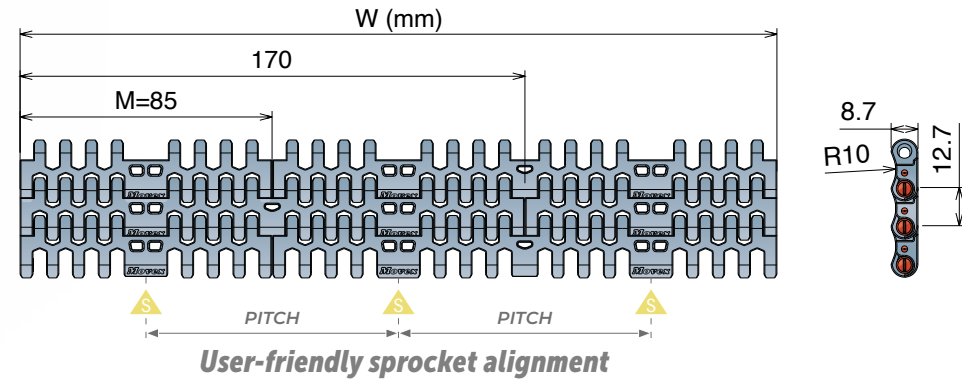
Version A - Standard
